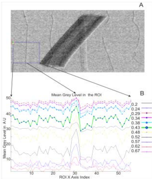
FIG. 3 MICRO WIRE PROFILES OBTAINED FOR A RANGE OF RECONSTRUCTED FREQUENCIES. SIGNAL PROFILES WERE EXTRACTED FROM A REGION OF INTEREST (ROI) AROUND A MICRO WIRE, INDICATED IN THE SQUARE LABELLED AS ‘1’ IN PANEL A. THE SIGNAL IS OBTAINED AS THE AVERAGE OVER THE LINES IN THE ROI, AND PLOTTED IN ABSOLUTE UNITS VERSUS PIXEL INDEXES ALONG THE ROI AS SHOWN IN B.
