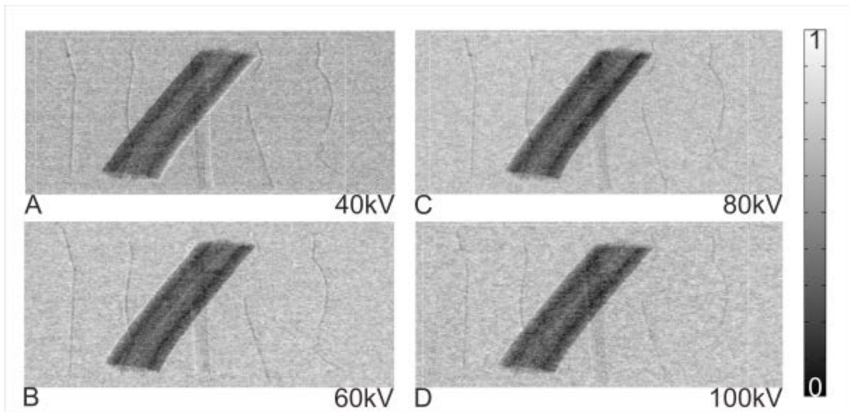
FIG. 1 X-RAY PHASE CONTRAST IMAGES OF THE CUSTOM BUILT PHANTOM SIMULATING A PLASTIC EXPLOSIVE DEVICE PLUS VARIOUS BINDING FIBRES AND THIN METALLIC WIRES (SEE TEXT). IMAGES A, B, C AND D WERE ACQUIRED AT INCREASING X-RAY TUBE VOLTAGES, AS LABELLED.
