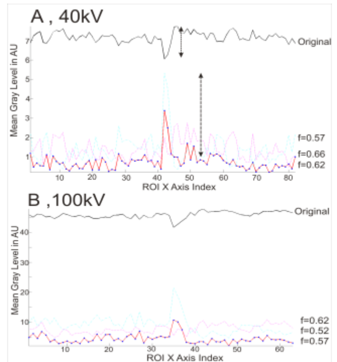
FIG. 4 A COMPARISON OF CONTRAST ENHANCEMENT IN THE SELECTED REGION OF INTEREST, FOR PROCESSED AND UNPROCESSED IMAGES, AT TWO DIFFERENT IMAGING CONDITIONS I.E. TUBE VOLTAGES OF 40 AND 100 KVP. THE PROFILES OBTAINED FROM IMAGES ARE PRESENTED FOR A RANGE OF FREQUENCIES f . THE FREQUENCY RANGE IS CENTRED AT THE MAXIMUM ENERGY IMAGE, AND VALUES ONE STEP BELOW AND ONE ABOVE IN THE FILTERBANK ( F_{EMAX-1}, F_{EMAX}, F_{EMAX+1} ) ARE ALSO SHOWN. A AND B SHOW PROFILES FROM IMAGES ORIGINALLY ACQUIRED AT 40 AND 100 KVP RESPECTIVELY, AND IN BOTH CASES A CONTRAST ENHANCEMENT OF THE ORDER OF \sim 300\% IS OBSERVED.
