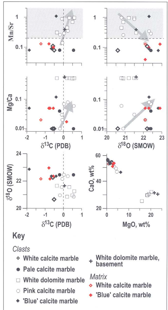
Fig. 17. Cross-plots showing the composition of different clast lithologies and matrix. Samples in the shaded areas are considered to have been subjected to alteration, i.e., with a Mn/Sr ratio > 0.2. Arrows indicate alteration trend caused by dolomitisation.
