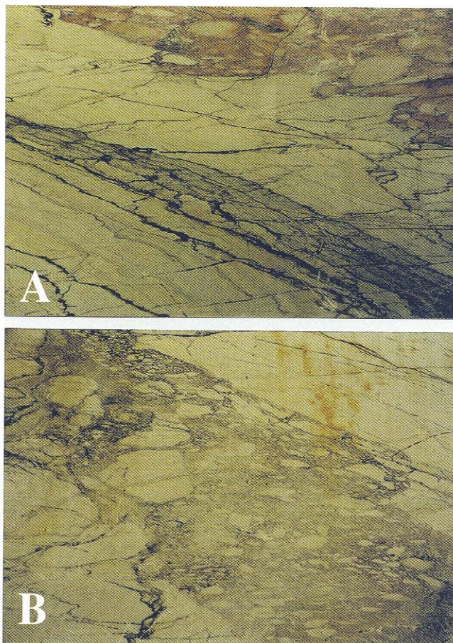
Fig. 5. The substrate to the Fauske conglomerate. (a) Banded, white to pale grey, dolomite marble with an irregular upper surface overlain by pink conglomerates. Note that the irregular palaeorelief beneath the conglomerate is strongly affected by the tectonic deformation, i.e., folding with a spaced cleavage forming the axial planes to mesoscopic folds. (b) An 'open' space between two large blocks of white dolomite marble filled with fragments of the same dolomite marble. The dolomite marble forms the substrate to the Fauske conglomerates. The photograph is taken 6 m below the contact with the conglomerates. Width of photographs = 2.5 m. Photographs taken from Channel 1, east face.
