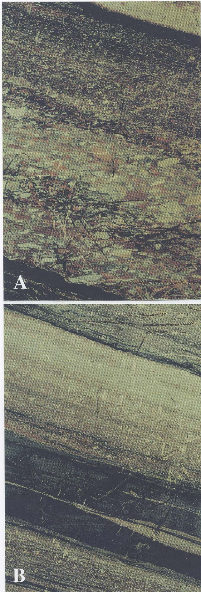
Fig. 8. Upward fining of clasts within individual beds. (a) Bed 14 exhibits four distinctive units which correspond to the A, B, C and D units of a typical Bouma sequence. The bed starts with a thick unit of conglomerobreccia overlain progressively by a fine-pebble conglomerate with parallel lamination, a thin unit of current-bedded gritstones, and at the top by a silty greywacke with plane-parallel lamination. Height of photograph = 1.2 m. (b) Lower part of Bed 18 (above the dark grey greywacke layer) exhibiting graded bedding accompanied by the development of an internal planar lamination. Height of photograph = 2.5 m. Both photographs taken from Channel 3, east face.
