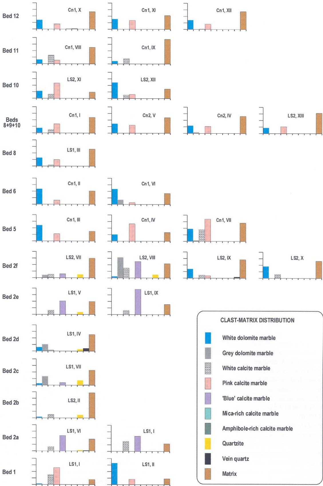
Fig. 15. Composition of clasts and matrices measured from different beds. The following abbreviations are used in the figure: Ch1 - Channel 1, Ch2 - Channel 2, LS1 - Longitudinal Section 1, LS2 - Longitudinal Section 2. Roman numerals indicate the section number which was used to count pebble composition; these sections are marked on Plates 1 and 2. Detailed logs of LS1 and LS2 are not presented in the article but they may be obtained from the first author on request.
