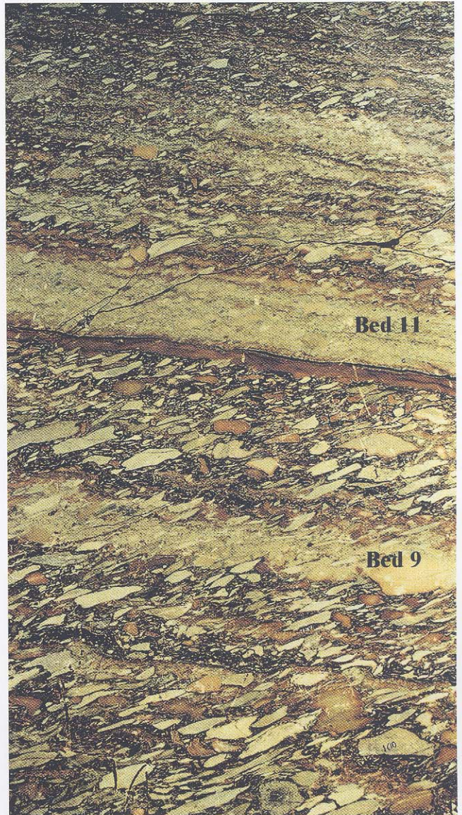
Fig. 9. Originally horizontally bedded carbonate breccia showing a gradual upward decrease in fragment size accompanied by the gradual development of an internal planar lamination; Beds 8-12. Note that Beds 9 and 11 are distinguished in the conglomerate sequence by their paler colours caused by a dominance of white dolostone fragments in a pale grey calcarenite matrix. The clasts are here (re)orientated within the D2 (S2) schistosity. Fault-related, proximal, submarine channel facies. Height of photograph = 2.5 m. Photographs taken from Channel 1, east face.
