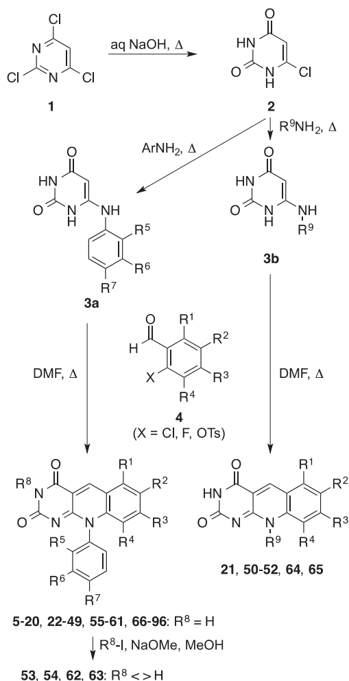
Scheme 1. Synthesis of 5-deazaflavin derivatives 5–96 . For definition of substituents R^{1-9} refer to Table 1.
