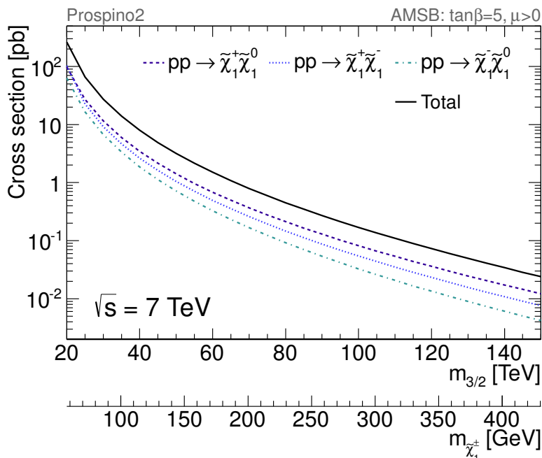
Figure 1. The cross-section for direct chargino production at \sqrt{s} = 7 \text{ TeV} as a function of m_{3/2} . The corresponding m_{\tilde{\chi}_1^\pm} values for each m_{3/2} are also indicated.
