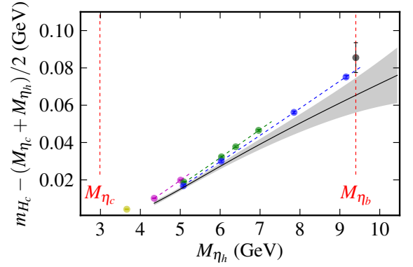
FIG. 4: Results for the mass difference between the H_c meson and the average of the associated heavyonium pseudoscalar meson masses plotted as a function of the pseudoscalar heavyonium mass. The lattice QCD results have been adjusted for slight mistuning of the c quark mass. The color scheme is as in Figure 1. The black circle with error bar at M_{\eta_b} gives the experimental value adjusted for the effects from electromagnetism, \eta_b/\eta_c annihilation and c quarks in the sea, none of which is included in the lattice QCD calculation.
