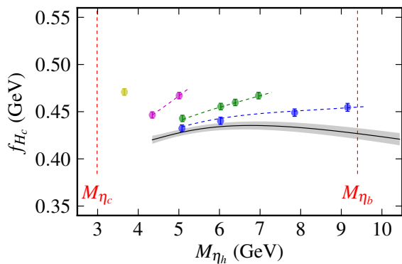
FIG. 7: Results for the heavy-charm decay constant plotted as a function of the pseudoscalar heavyonium mass. The lattice QCD results have been adjusted for slight mistuning of the c quark mass. The color scheme is as in Figure 1.
