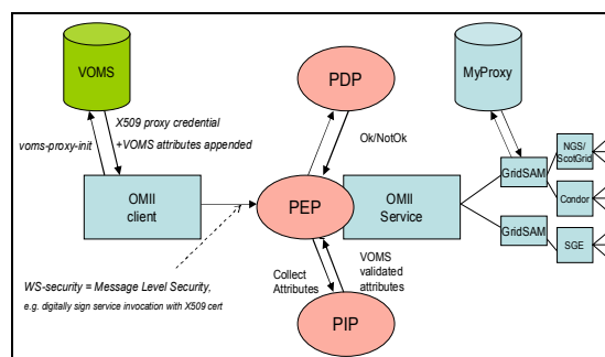
Figure 2: OMII-UK VOMS-PERMIS Integration
