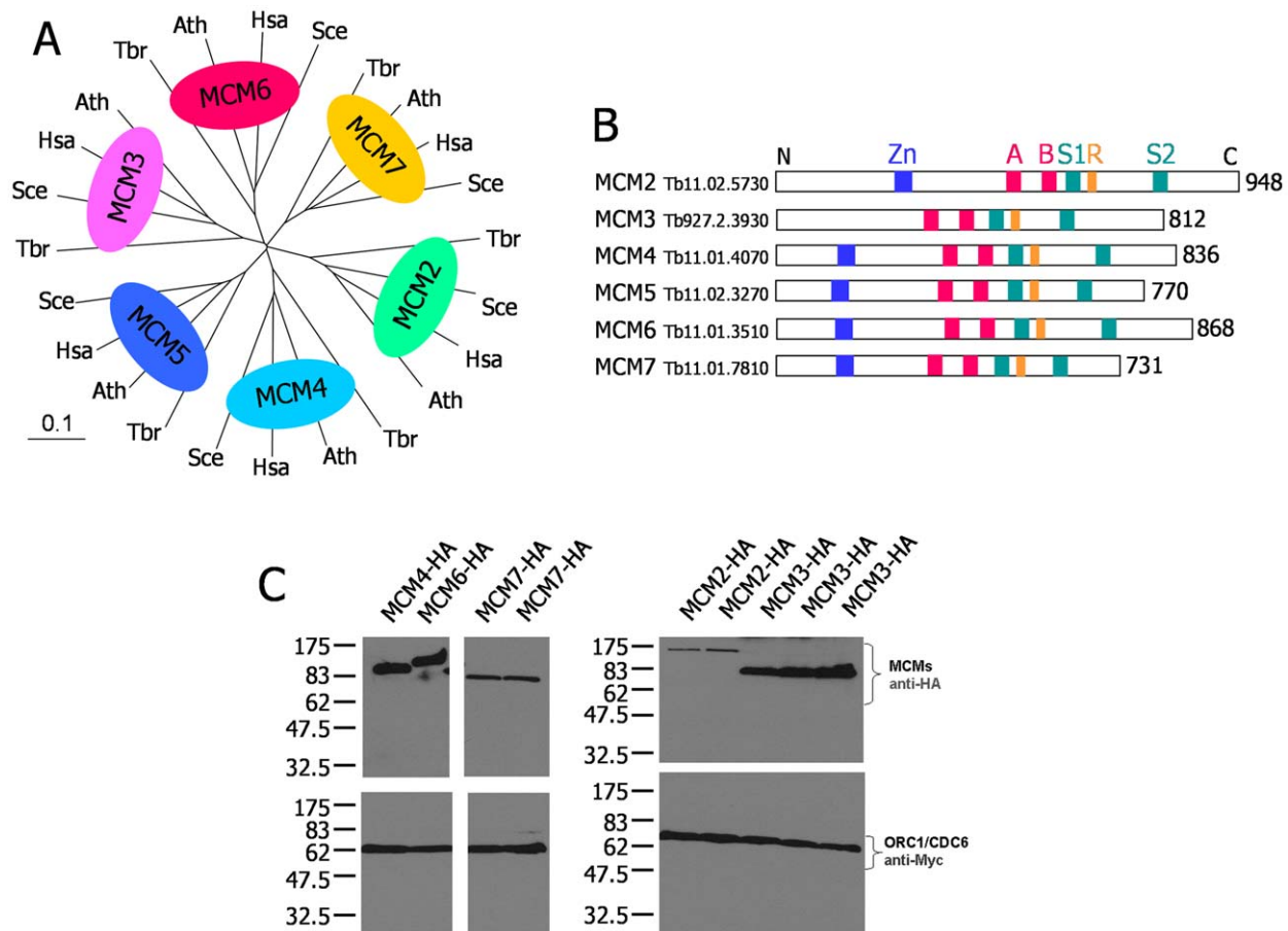
Figure 1. MCM helicase subunits in T. brucei and co-expression with ORC1/CDC6 as epitope tagged variants. A. An unrooted phylogenetic tree is shown, detailing the homology between predicted MCM helicase subunits in T. brucei (Tbr) relative to orthologues in H. sapiens (Hsa), S. cerevisiae (Sce) and A. thaliana (Ath). Complete protein sequences were aligned with ClustalX, using default settings, and the phylogenetic tree was displayed using TreeView (Page, 1996); the distance corresponding to 10 amino acid changes per 100 positions is indicated (0.1). B. A diagrammatic representation of the MCM helicase subunits in T. brucei . The length of the predicted polypeptides is shown (in amino acid residues), and the position of conserved functional motifs are indicated: an N-terminal Zinc Finger (Zn, blue box); and Walker A and B boxes (A and B, red boxes), an Arginine finger (R, orange box) and sensor 1 and 2 motifs (S1 and S2, green boxes), all involved in nucleotide binding and hydrolysis. C. Western blots of procyclic form TREU 927 T. brucei cells co-expressing C-terminally HA-tagged TbMCM subunits (MCM-HA) and C-terminally Myc-tagged TbORC1/CDC6. The upper panel shows TbMCM-HA expression in whole cell extracts, detected using anti-HA antibody, and the bottom panel shows TbORC1/CDC6-Myc from the same whole cell extracts detected using anti-Myc antibody. Single clones are shown for TbMCM4-HA and TbMCM6-HA, two clones for TbMCM2-HA and TbMCM7-HA, and three clones for TbMCM3-HA. Size markers (kDa) are indicated. doi:10.1371/journal.pone.0032674.g001
