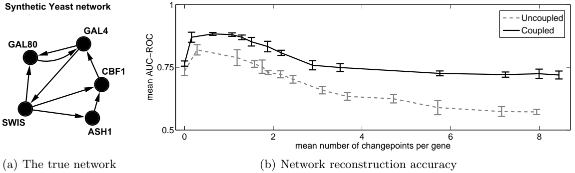
Figure 3: Gene network reconstruction accuracy for the S. cerevisiae data. Cantone et al. (2009) designed the network shown in panel a) and measured in vivo gene expression levels with RT-PCR. The graph shows the network reconstruction accuracy (ordinate) plotted against the mean number of changepoints per gene (abscissa) for the conventional uncoupled (dashed) and the proposed coupled NH-DBN (solid line). The network reconstruction accuracy is quantified in terms of mean AUC-ROC scores, averaged over 5 MCMC simulations, with the vertical bars indicating standard errors. A similar plot with AUC-PR scores is provided in the supplementary material.
