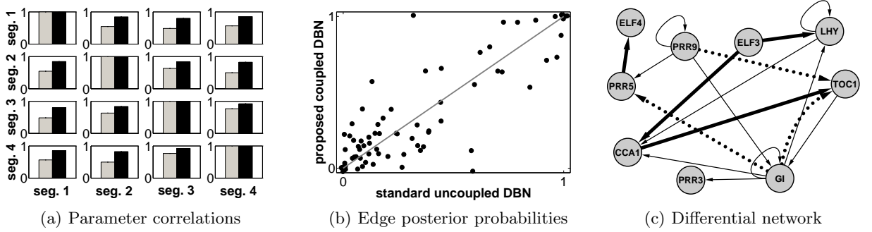
Figure 2: Inference for the A. thaliana gene expression time series. a) Histograms of the average similarities (correlations) of the interaction parameters, sampled from the posterior distribution with MCMC between four time series segments, indicated by the rows and columns. Details on the segmentation can be found in Subsection 4.2. The networks were sampled from the posterior distribution, see (23), with MCMC. Each panel contains a histogram that shows the average similarity of the interaction parameters among segments for the conventional uncoupled (grey) and the proposed coupled (black bars) NH-DBN; see main text for details on our similarity measure. b) Scatter plot of the marginal edge posterior probabilities inferred with the uncoupled (horizontal) and the coupled (vertical axis) NH-DBN. c) The (differential) network prediction that can be obtained when the threshold 0.75 is imposed on the edge posterior probabilities. Thin black edges indicate interactions that are inferred with both NH-DBNs. Three edges (dotted) are inferred with the conventional NH-DBN only while four edges (bold) are inferred with the coupled NH-DBN only.
