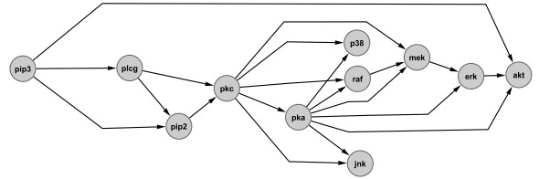
(a) The RAF network (Sachs et al. , 2005)
