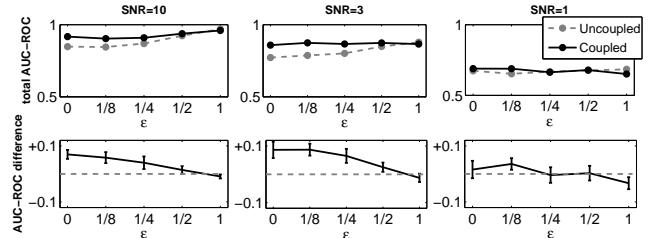
(b) Network reconstruction accuracy for the RAF network
