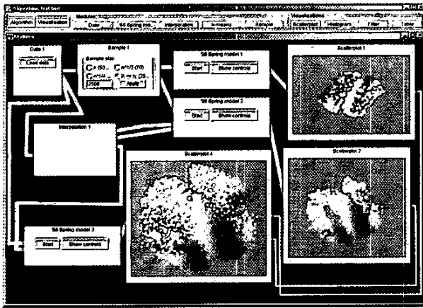
Figure 1. Two screen-shots of the HIVE interface. The image on the left illustrates interconnected components that import, transform and render multidimensional data. The algorithmic components collectively represent the O(N^2N) hybrid MDS algorithm of [Morrison et al. 2002]. Thick lines that link modules represent data-flows while thin ones, connecting scatterplots and other visualisations, represent the connections between interlinked interactive views. The image on the right shows the same scatterplots enlarged and supplemented with a fisheye table component. The data consists of 5000 points sampled from a 3D 'S' shaped distribution.
