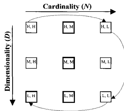
Figure 2. Data input to components in a hybrid algorithmic architecture can be categorised by the ranges of dimensionality and cardinality they are best suited for—high, medium or low. Each component transforms the data, effectively moving across the 3x3 grid. Our hybrid layout algorithm produces a low-dimensional layout of a large high-dimensional data set i.e. a move from (H,H) to (L,H) that involves several steps shown as dotted lines in the figure: sampling, which reduces N , then a spring model of the sample, which reduces D , and then interpolation, which increases N .
