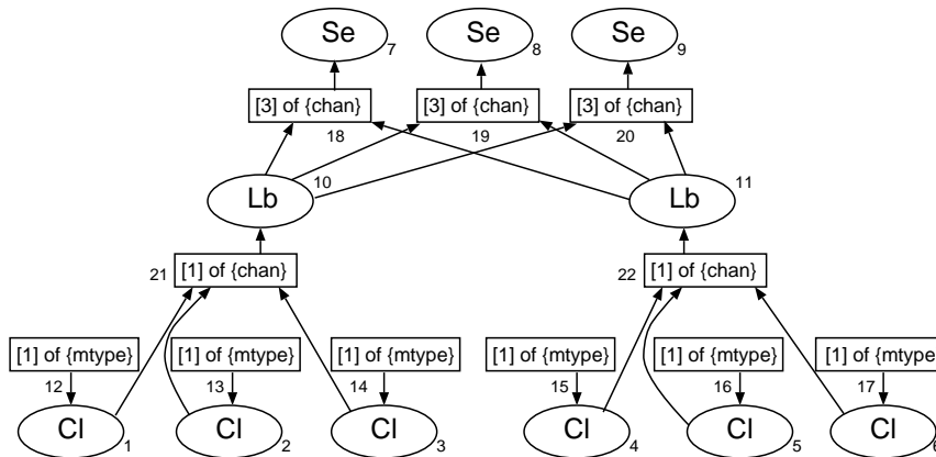
Fig. 1. Channel diagram of the load balancing example—clients are denoted Cl, servers Se and load balancers Lb.
