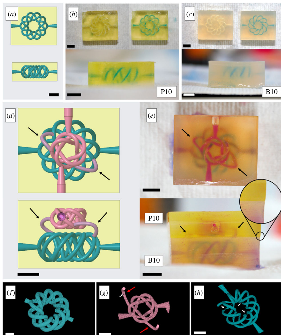
Figure 4. (a) CAD file of a (3,10) torus knot converted into a microvascular structure in PEGDA10 from the front and top views. (b) and (c) three-dimensional printed microvasculature in PEGDA10 and BEMA10, respectively, showing the empty and filled channels. (d) CAD file of two interconnected (3,10) and (3,5) torus knots (from the top and front views). Arrows indicate the parametric curves that connect the top torus knot (representing the solid tumour's vasculature) with the bottom torus knot (representing healthy vasculature). (e) Top and front views of the multi-material three-dimensional printed interconnected (3,10) and (3,5) torus knots. The arrows indicate the simplified replica of the neo-vasculature, where fluid migrates from the diseased-mimicking vasculature to the healthy-mimicking vasculature. The circle close-up shows the transition from BEMA10 to PEGDA10. Scale bars = 5 mm. (f) \mu CT reconstruction of the single-material three-dimensional printed (3,10) torus knot. Scale bar, 2.5 mm. (g) and (h) \mu CT reconstructions of the (3,5) and (3,10) torus knots, respectively. White arrows indicate small volumes of air trapped in the lead-loaded resin, and red arrows indicate the neo-vasculature. Scale bars = 1 mm.
