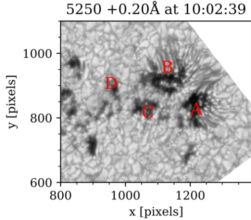
Figure 3. Fe I 5250 Å image showing the underlying sunspots and pores of the active region. The largest sunspots are labelled as they will be referred to throughout this paper.
