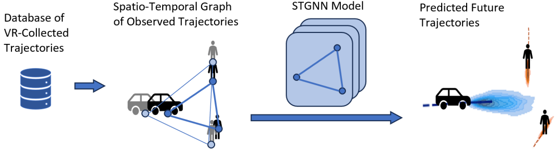
Figure 6: Overview of the STGCNN architecture and how it has been integrated in our system. The data collected with the VR equipment is processed and the STGCNN provides predictions of future trajectories.
