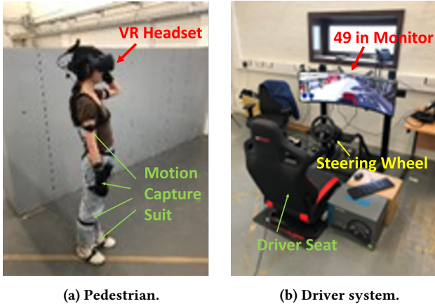
Figure 3: a) A pedestrian wearing the VR and Motion Capture system, b) the driver setup.
