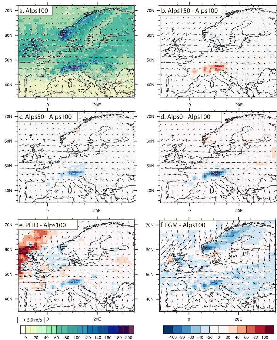
Figure 3. (a) ECHAM5-simulated mean summer (JJA) precipitation amount for the preindustrial (Alps100) experiment (mm/month) and winds at 10 m. Calculated precipitation differences for (b) Alps150 – Alps100 and Alps150 winds at 10 m, (c) Alps50 – Alps100 and Alps50 winds at 10 m, (d) Alps0 – Alps100 and Alps0 winds at 10 m, (e) PLIO – Alps100 and PLIO winds at 10 m, and (f) LGM – Alps100 and LGM winds at 10 m. Isolines on subplot (a) show topography for Alps100 experiment; isolines from 500 m, with a 500-m contour interval.
