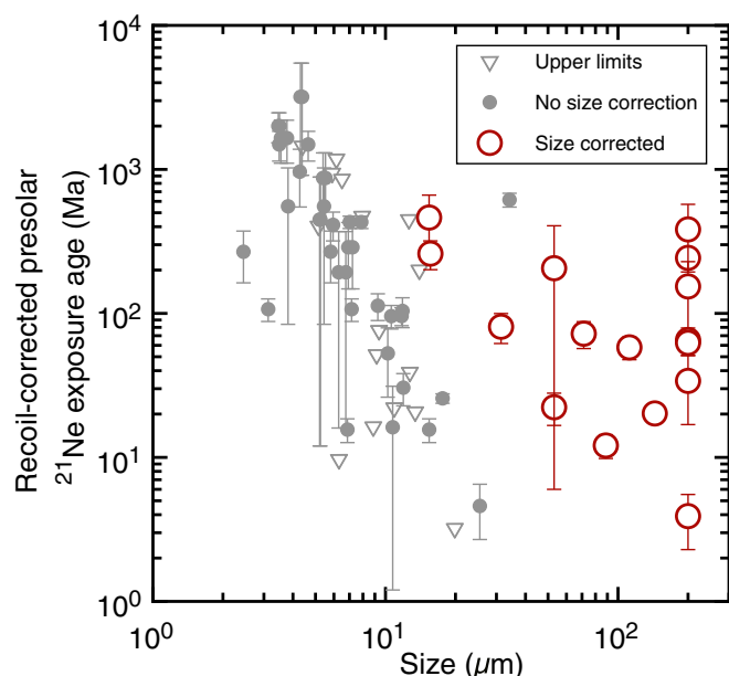
Fig. 4. Older grains are smaller. Size is given as the geometric mean of the diameter of the grains. Size-corrected data are for aggregates during irradiation in the ISM. Aggregates of >200\ \mu\text{m} are shown at 200\ \mu\text{m} . Size measurements of all grains are given in SI Appendix .
