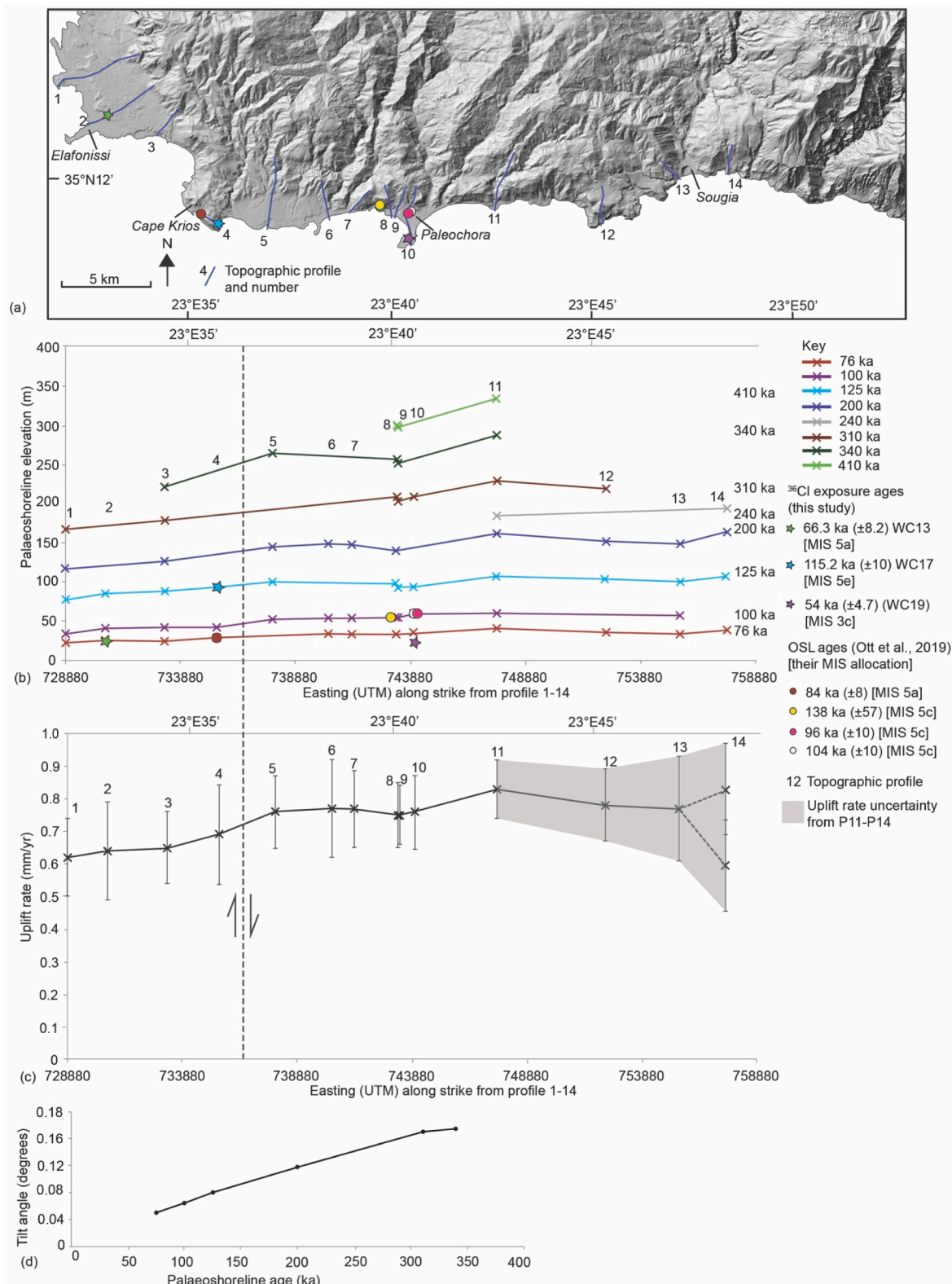
Fig. 8. (a) DEM showing the locations of profiles, 36 Cl exposure ages and OSL ages (Ott et al., 2019). (b) Along strike palaeoshoreline elevations for sea-level highstands from 76 ka to 410 ka showing an elevation increasing from P1 in the west to P11 in the east. (c) Uplift rates obtained from analyses of the topographic profiles in Fig. 7. Note that for P14, two uplift rate scenarios are illustrated (see Table 3). Uplift rate uncertainty is illustrated from P11–P14 because of a lack of age controls and the two possible uplift rate scenarios at P14. Dashed line is the location of a localised fault (Ott et al., 2019) suggested to exist between P4 and P5, see text for discussion (d) Tilt angles for each palaeoshoreline show that older palaeoshorelines are more tilted than younger palaeoshorelines. The tilt angles are calculated using the length of each palaeoshoreline from the lowest uplift location profile (P1) to the highest uplift location profile (P11) and the change in elevation from P1–P11. Note that tilt angles for the 240 ka and 410 ka palaeoshorelines cannot be calculated owing to a lack of along strike measurements.
