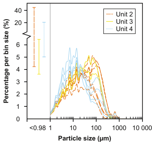
Fig. 7. Particle-size distribution data illustrated as percentage per bin. The data are binned as frequency per 1/4 phi unit. Particle size <0.98 is given as percentage range per Unit.
