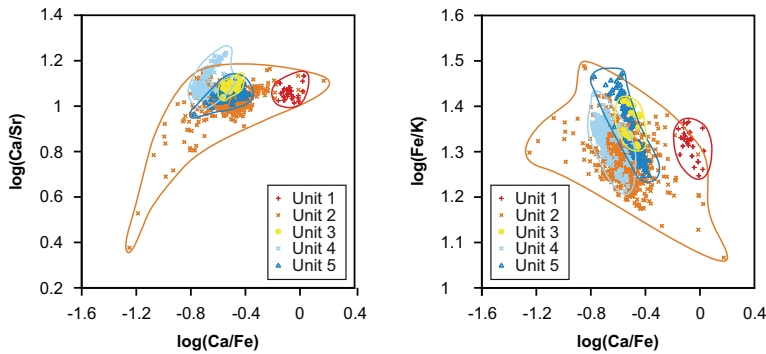
Fig. 6. ITRAX XRF composition of individual subunits compared as cross plots. Red crosses, Unit 1; orange crosses, Unit 2; yellow circles, Unit 3; light blue stars, Unit 4; dark blue triangles, Unit 5.
