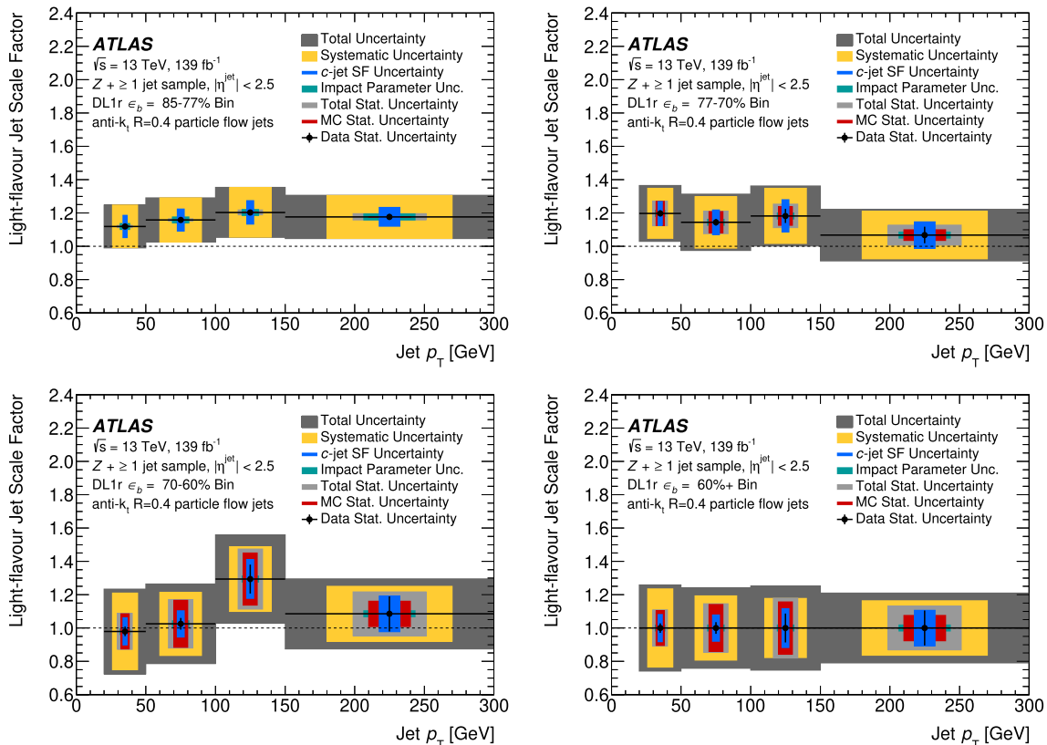
Fig. 7 SFs to calibrate the \varepsilon^{\text{light}} of the pseudo-continuous OPs. The size of the uncertainty bands in the direction of the jet p_T axis is arbitrary and corresponds to the choice of the calibration intervals in p_T
