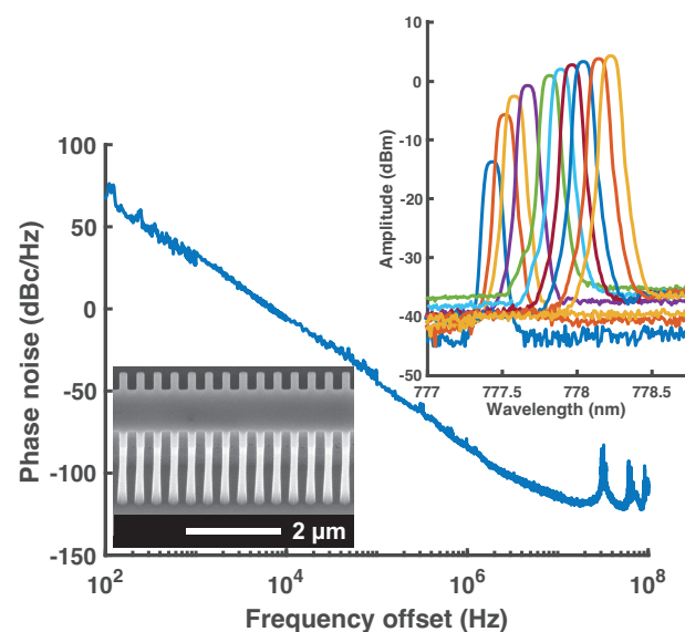
Fig. 2. The phase noise of a free-running 778.1 nm DFB laser as a function of offset frequency providing a Lorentzian linewidth of 3.7 kHz over 25 \mu\text{s} integration time. Insert left: A SEM image of the DFB grating. Insert right: The laser output amplitude when the current is tuned from 120 mA to 300 mA in 20 mA steps.
