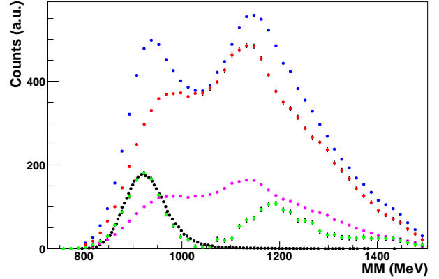
FIG. 9: Subtraction of the carbon background for proton events using the missing mass plots obtained from D-butanol and carbon data for W (total center-of-mass energy) between 1450 and 1480 MeV. The different points represent the missing mass distribution for: the D-butanol target (blue dots), the carbon target (magenta dots), the scaled carbon (red dots) and the proton events (green dots) obtained by subtracting the scaled carbon events from the D-butanol events. The black dots show the simulated distribution of quasi-free proton events from a deuterium target.
