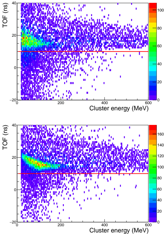
FIG. 6: ToF analysis for neutral (top) and charged (bottom) tracks after the PSA cut. The neutron and proton candidates lying below the red lines have been rejected.
