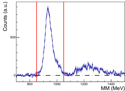
FIG. 3: Missing mass (MM) distribution for the sum (top) and the difference (bottom) of events obtained with the parallel and anti-parallel photon-target helicity configurations. The acceptance region for the N\pi^0 events is inside the red vertical lines at MM = 850 and 1050 MeV. The background evident in the right tail of the MM distribution comes from the \pi^0\pi^0 and the \pi^0\pi^\pm channels.
