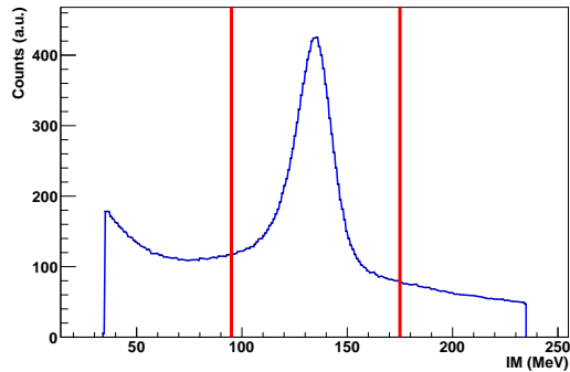
FIG. 2: Two photon invariant mass (IM) distribution from the \pi^0 reconstruction procedure for all candidate events. The red lines define the \pm 40 MeV cut (corresponding to an experimental resolution of about 2.5 \sigma ) around the nominal m_{\pi^0} value.
