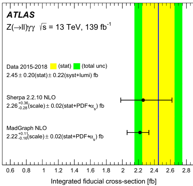
Fig. 4 The Z(\rightarrow ll)\gamma\gamma integrated cross-section, measured in a fiducial region corresponding to the production of three on-shell electroweak bosons. The measurement is compared with both the signal event generator predictions
