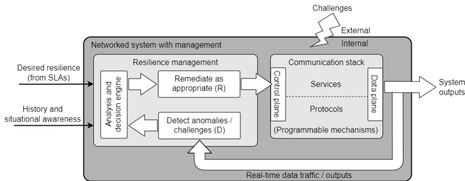
Fig. 2. A resilience control loop: derived from the real-time component of the D^2R^2+DR resilience strategy (see chapter 1 in [1])
