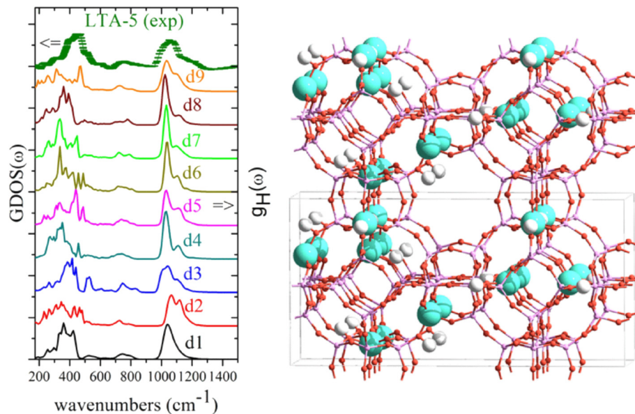
Fig. 3 Left: Comparison between the experimental INS spectrum of LTA-5 (a specially synthesised high-silica form of LTA with Si:Al = 5) and the hydrogen partial density of states, g_H(\omega) , of the fundamental vibrations calculated by periodic DFT for the models of the possible Brønsted acid site locations. Right: “d5” the structure that produces the spectrum that best matches the INS results. Note that the hydroxyls are distributed relatively far from each other. The figure has been reproduced from ref. 59 with permission from Elsevier, copyright 2013.
