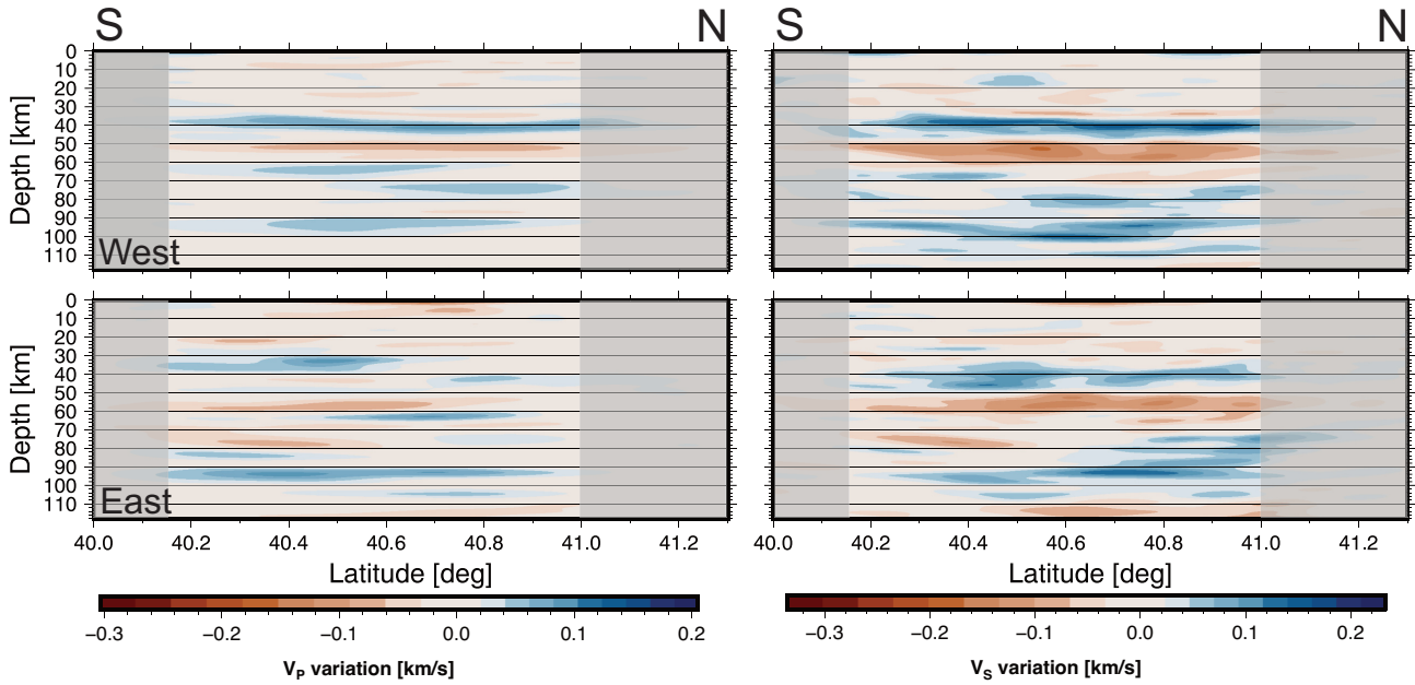
Figure 10. North–south depth slices of the model stacked in longitude (a) for dV_P and (b) dV_S . Top figure for each velocity variation is for the western section (west of 30.4^\circ\text{E} ) of the model with the bottom the eastern part (east of 30.4^\circ\text{E} ).
