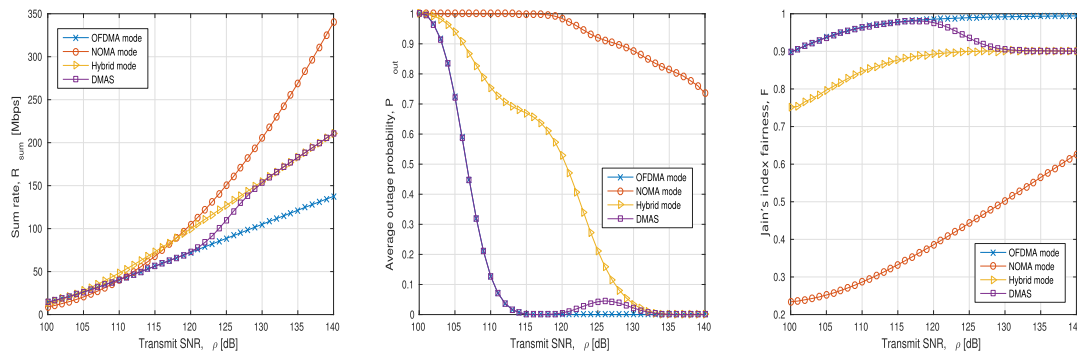
FIGURE 7. Achieved performance under the different MA schemes compared to the proposed DMAS with [\omega_{R_{sum}}, \omega_{P_{out}}, \omega_{\mathcal{F}}] = [0.4, 0.3, 0.3] for a system with 6 multiplexed users.
