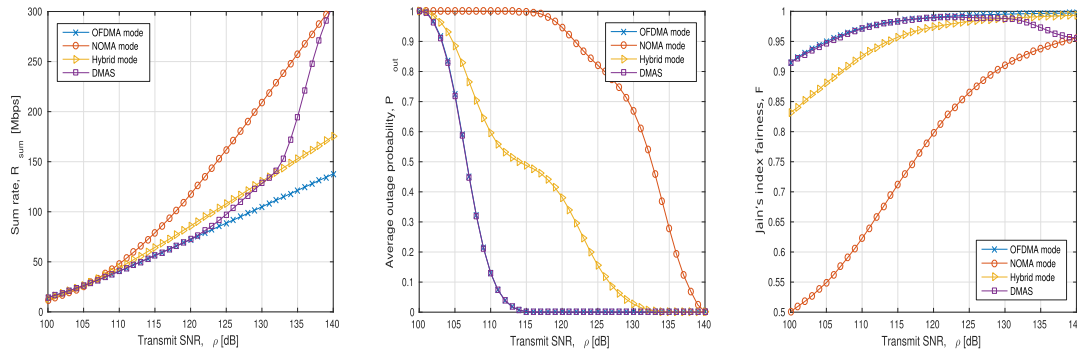
FIGURE 6. Achieved performance under the different MA schemes compared to the proposed DMAS with [\omega_{R_{sum}}, \omega_{P_{out}}, \omega_{\mathcal{F}}] = [0.4, 0.3, 0.3] for a system with 3 multiplexed users.
