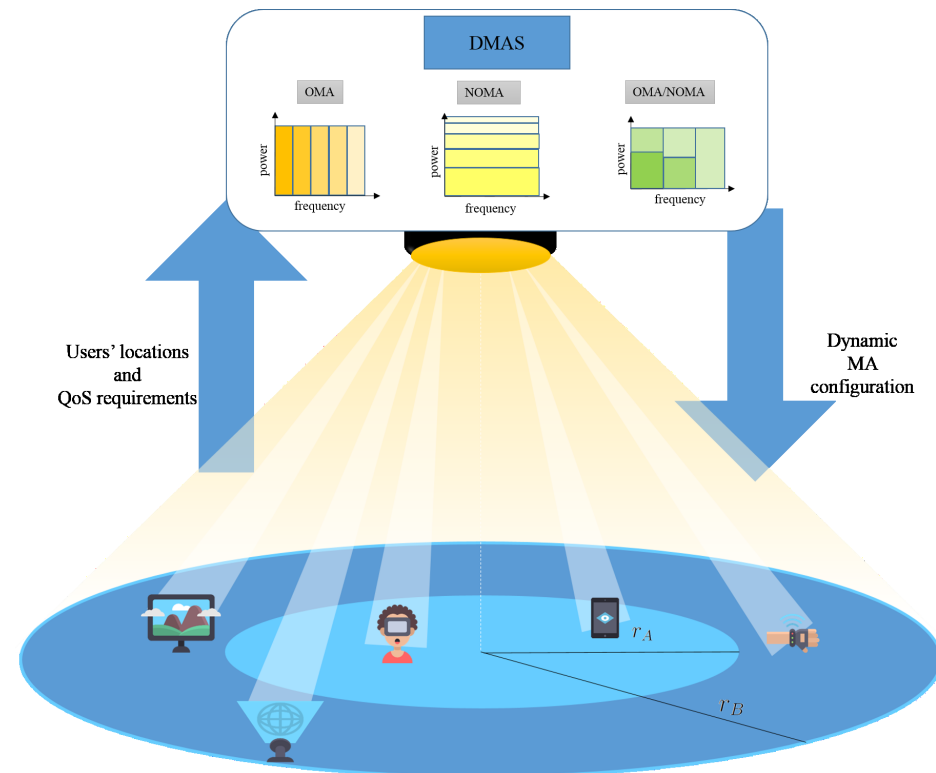
FIGURE 1. LiFi downlink framework.
