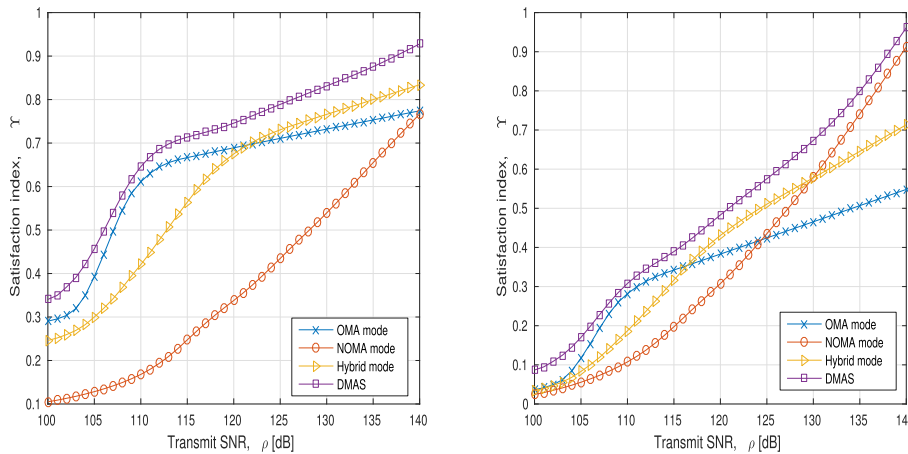
FIGURE 11. Satisfaction index of the proposed DMAS with (a) [\varpi_{R_{sum}}, \varpi_{P_{out}}, \varpi_{\mathcal{F}}] = [0.4, 0.3, 0.3] and (b) [\varpi_{R_{sum}}, \varpi_{P_{out}}, \varpi_{\mathcal{F}}] = [0.8, 0.2, 0] compared to the different MA modes.
