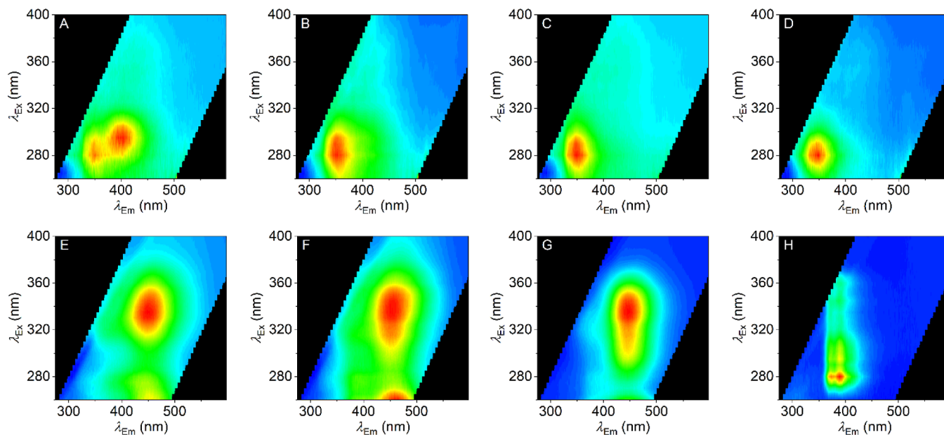
Figure 2. (A–D) FSFs for methanone-linked series of SCRA analogues 1a–d (A = 1a , B = 1b , C = 1c , and D = 1d ), collected prior to sample irradiation. (E–H) FSFs for ethanone-linked series of SCRA analogues 2a–d (E = 2a , F = 2b , G = 2c , and H = 2d ), collected prior to sample irradiation. Red coloration represents emission with a relative intensity of 1, and blue represents an intensity of 0. Conditions: 0.01 mg/mL in methanol, 20 °C, and 1 cm path length.
