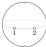
\ell = 2
