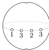
\ell = 3
