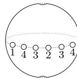
\ell = 4
