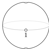
\ell = 1
