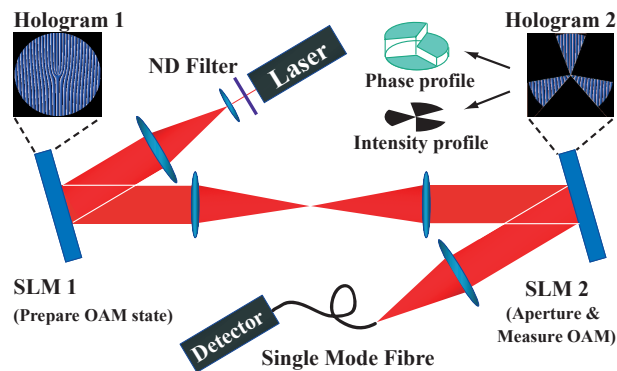
Fig. 1. Spatial light modulators are used to create specific OAM states (SLM1), aperture them and measure the resulting OAM distribution (SLM2).
