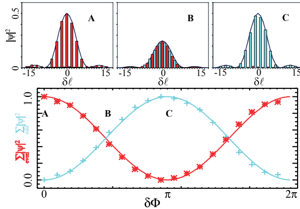
Fig. 3. Experimental result for two equi-spaced segment apertures of angular width 2\pi/9 . Panels A, B and C show the observed angular momentum spectra for \delta\Phi = 0, \pi/2 and \pi , respectively, with the predicted envelope function (solid line) and experimentally measured data (bars). Even sidebands are plotted in red and odd sidebands in cyan. The main panel shows the sums of coefficients of even (red) and odd (cyan) OAM sidebands as a function of phase difference, \delta\Phi , between the segments. Solid curves show the predicted variation.
