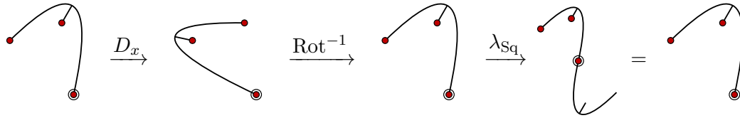
FIGURE 22. An invariant tree for D_x^{-1} R
