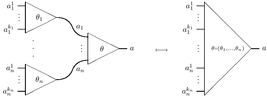
Figure 2-B: Composition in a multicategory
