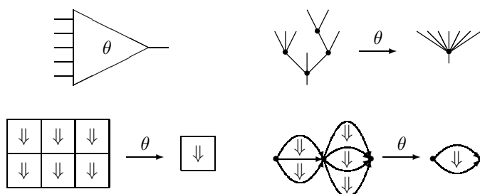
Figure 0-A: Operations \theta in four different types of generalized operad
