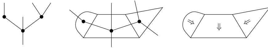
Figure 7-A: How a tree corresponds to a diagram of pasted-together 2-opetopes
