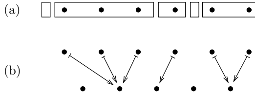
Figure 7-B: Two pictures of a map 6 \rightarrow 5 in \mathbb{D}
