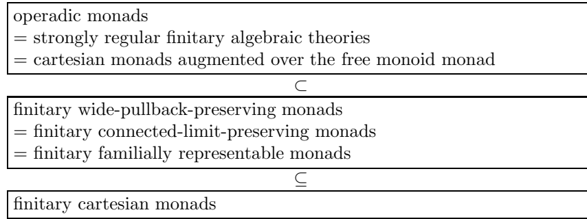
Figure C-A: Classes of finitary cartesian monads on Set
