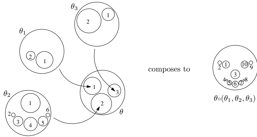
Figure 2-F: Window to Plato’s heaven
