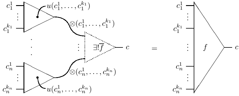
Figure 3-B: Representation of a multicategory
