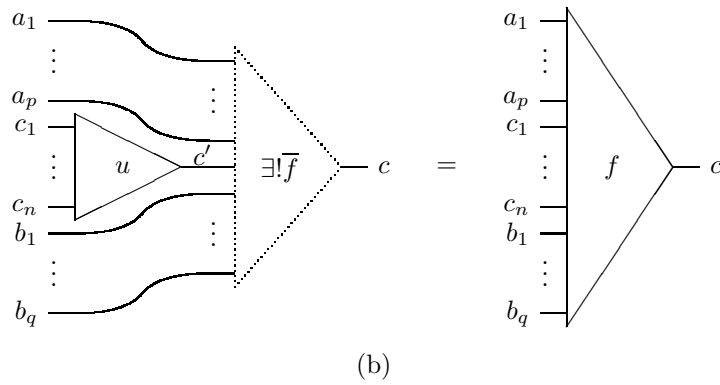
Figure 3-C: (a) Pre-universal map, and (b) universal map
