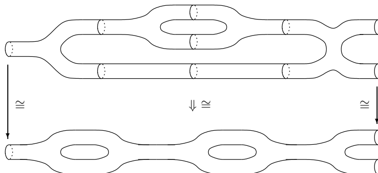
Figure 5-B: 2-cell in the fc -multicategory 1\text{-Mfd}_2 , with 4 horizontal 1-cells along the top row
