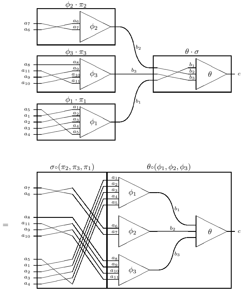
Figure 2-H: Symmetric multicategory axiom
