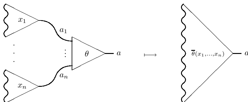
Figure 2-D: Action of a multicategory on an algebra
