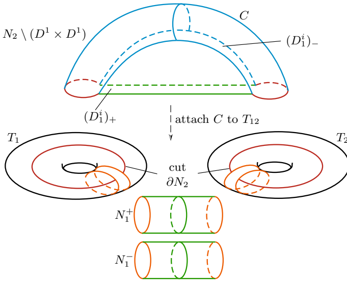
Fig. 5 Schematic diagram of the construction of the disc C from surgery on N_2 using D_1^i , and the construction of T_{12} from the Clifford tori T_1 and T_2 and two parallel copies N_1^\pm of the annulus N_1
