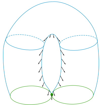
Fig. 6 The Whitney framing of the normal bundle of a Whitney disc along the boundary. It is tangent to \Sigma_1 , which appears in the picture as a plane, but normal to the \Sigma_2 , which is the surface that appears as a line in the picture
