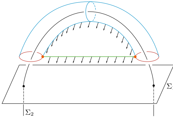
Fig. 6 The Whitney framing of the normal bundle of a Whitney disc along the boundary. It is tangent to \Sigma_1 , which appears in the picture as a plane, but normal to the \Sigma_2 , which is the surface that appears as a line in the picture
