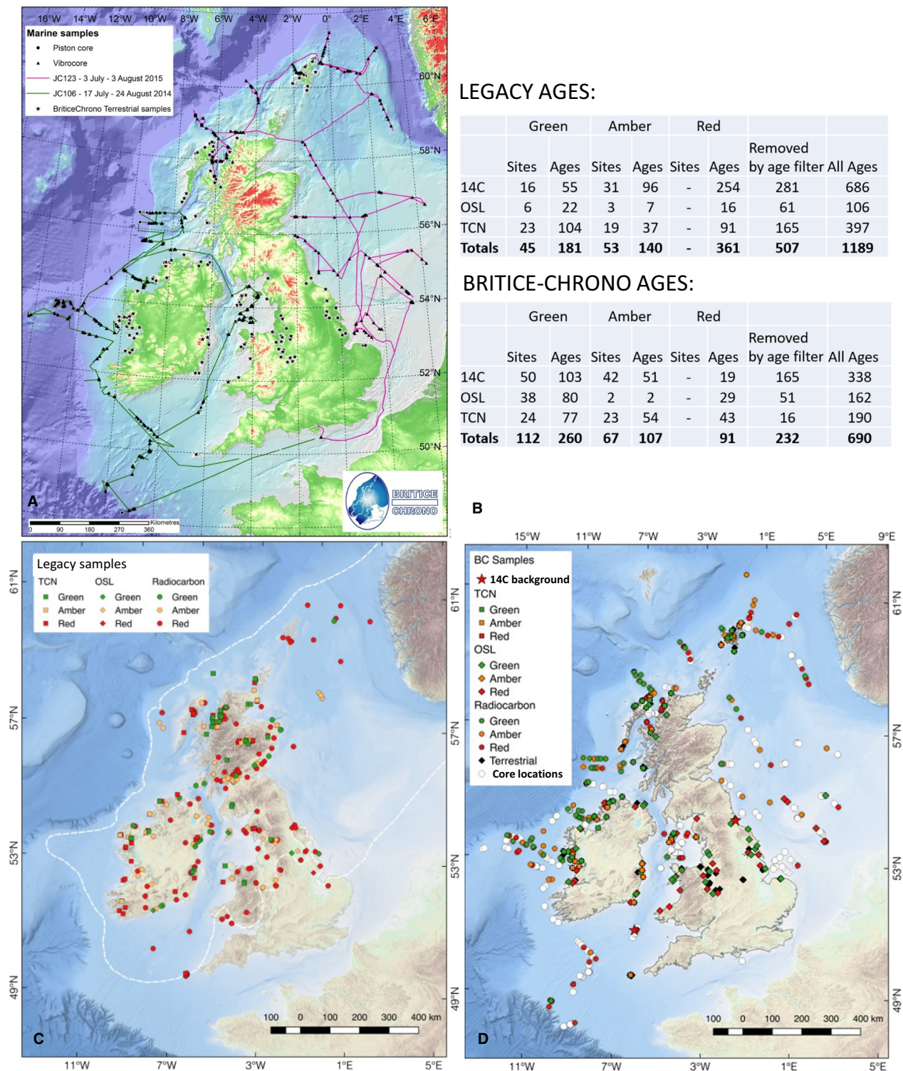
Fig. 2. A. Distribution of the BRITICE-CHRONO samples collected for dating, spread across 914 sites. Seabed samples were collected by vibro and piston corers from two research cruises in 2014 (green) and 2015 (purple). Terrestrial samples (asterisks) were collected for the immediately onshore zones of each transect in order to capture the pace of the ice margin retreat once it back-stepped onshore. B. Summary table and maps of age constraints from the (C) Legacy archive and (D) BRITICE-CHRONO databases. See text for details of the red, amber and green quality designators. The full Legacy database is available in Small et al. (2017b) and the BRITICE-CHRONO database in Data S2, this paper.
