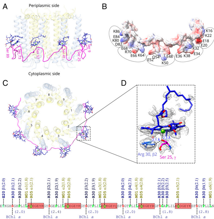
Fig. 4. Interaction of the \gamma -polypeptide with the surface of PucD-LH2. (A) Side view of the \gamma -subunit, which is enhanced by fading the \alpha/\beta -helices. Serine residues that ligand to BChls are labeled. (B) Electrostatic representation of the \gamma -polypeptide, which was rotated 45^\circ relative to A. Twenty charged residues, facing toward the cytoplasmic side, are shown as five groups outlined by dashed ellipses. (C) Top view of the \gamma -subunit from the periplasmic side of the complex. (D) A selected serine residue that coordinates the central Mg^{2+} of BChl and interacts with \alpha/\beta -helices through an H bond. (E) A map of the primary sequence of the \gamma -polypeptide. Residues involved in H bonds are in green. Serine residues coordinating BChl are in red. Bond lengths in angstroms are included in parentheses. Highlighted regions are the charged residue groups shown in B.
