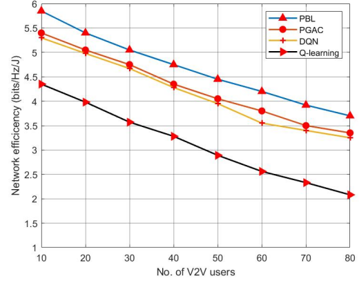
Fig. 2: Composite efficiency against number of V2V users.
