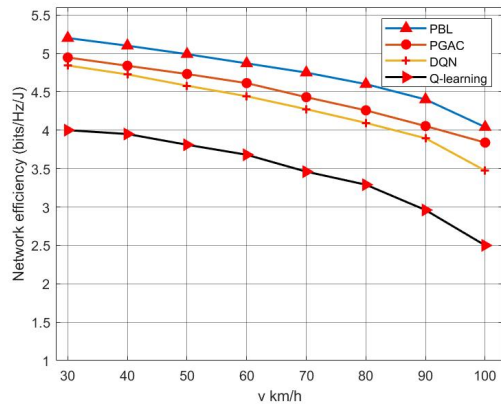
Fig. 4: Network efficiency with varying speed.
