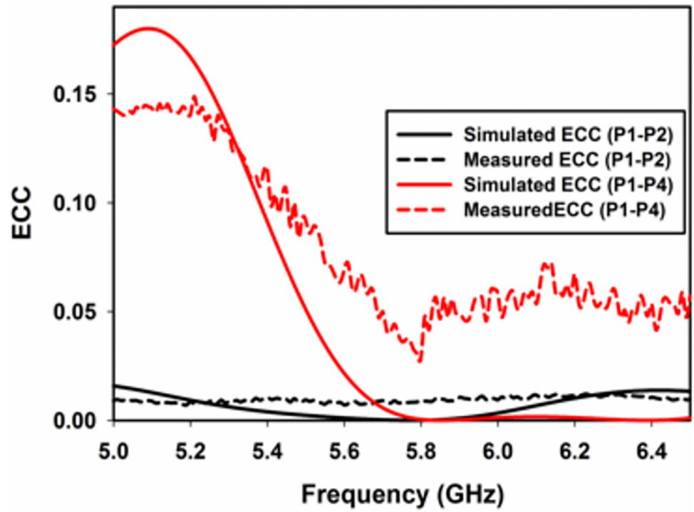
Fig 13. Simulated and measured ECC.
