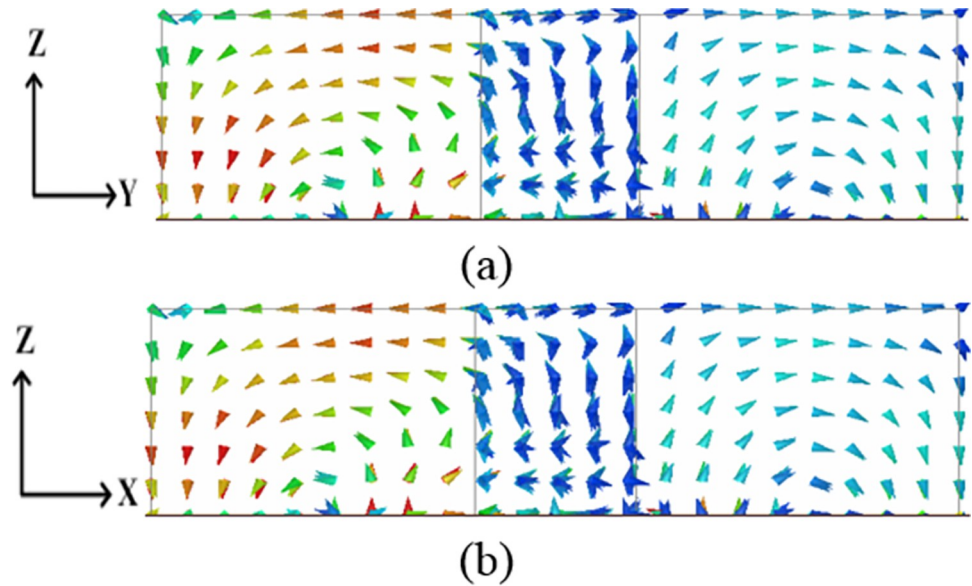
Fig 2. Patterns of electric field distribution (a) TE_{221}^x mode at 5.8 GHz and (b) TE_{221}^y mode at 5.8 GHz.
