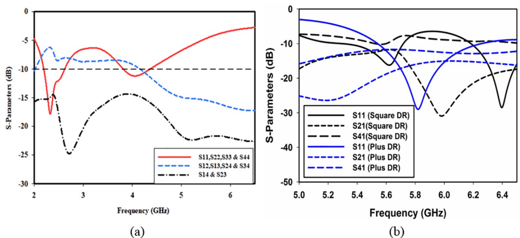
Fig 3. Input reflection (a) without DR and (b) with DR.
