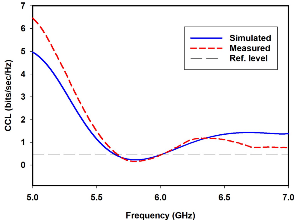
Fig 16. Simulated and measured CCL.
