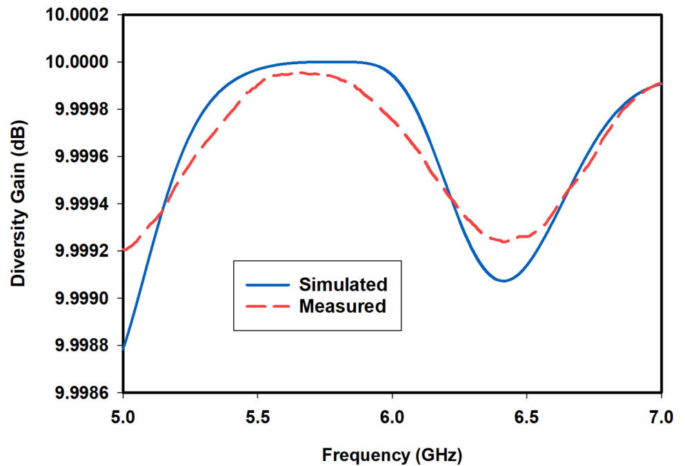
Fig 14. Simulated and measured DG.
