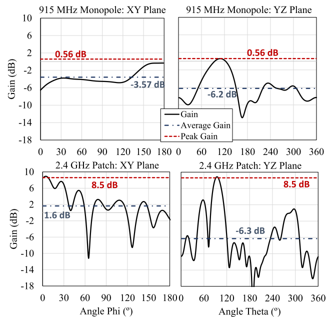
FIGURE 10. The patch and monopole antennas gain as a function of the angles \theta and \phi , as well as the peak and average (mean) gains over each plane.
