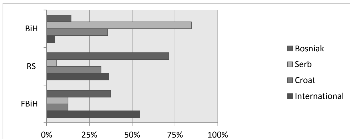
Figure 1. Percentage of Votes for a Constitutional Violation in Abstract Review Decisions
