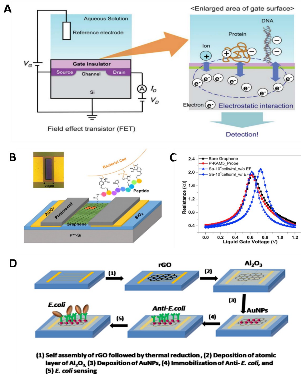
Figure 5: A. Basic Design and Operation of a FET-based sensor. [81] (Reproduced from reference [81] with permission. Copyright 2013 RSC); B. Design of the G-FET proposed by Kumar and associates; C. Distinct change in variation of resistance with liquid gate voltage with the G-FET and 10^4 SA cells/mL. [82] (Reproduced from reference [82] with permission. Copyright 2020 Elsevier); D. Schematic showing the design of the FET sensor proposed by Thakur et al. [84] (Reproduced from reference [84] with permission. Copyright 2018 Elsevier)
