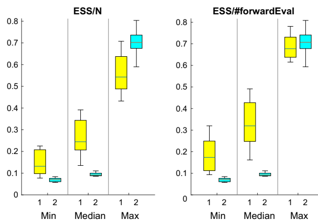
Fig. 7 Efficiency in terms of ESS of the algorithms compared (1: DA-GP-HMC, 2: DA-GP-NUTS) for the biochemical pathway example. Min, median, max ESS were calculated using Eq. (13). We show the distribution over 10 data sets. Legend: HMC—Hamiltonian Monte Carlo, NUTS: No U-turn sampler, DA—delayed acceptance, GP: Gaussian process, ESS: effective sample size, N—number of total MCMC samples, #forwardEval—number of forward simulations from the ODE model. See Table 1 for further explanations of the abbreviations
