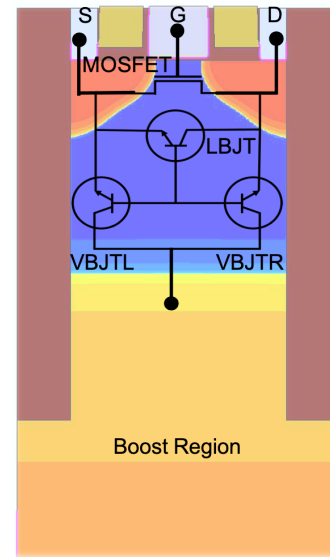
Fig. 1. The 1T SRAM cell structure (28 nm bulk CMOS technology) with an overlay showing the different built-in transistors. VBJTL and VBJTR are the left and right vertical BJTs, and LBJT refers to the lateral BJT.
