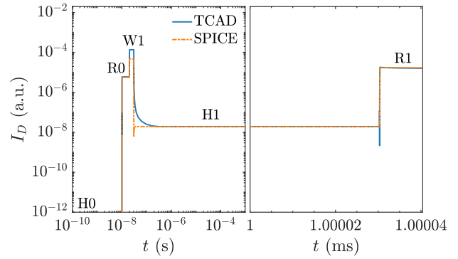
Fig. 8. TCAD Vs SPICE: current waveforms for the full operation of the 1T SRAM cell for illustration purposes with prolonged H1 and R1 to demonstrate stability. HO: HOLD ‘0’, R0: READ ‘0’, W1: WRITE ‘1’, H1: HOLD ‘1’, R1: READ ‘1’. Note the different time scales used in the two halves of the figure in order to properly display the relevant transitions regions.
