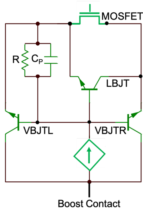
Fig. 4. The 1T SRAM cell's equivalent circuit macro model.
