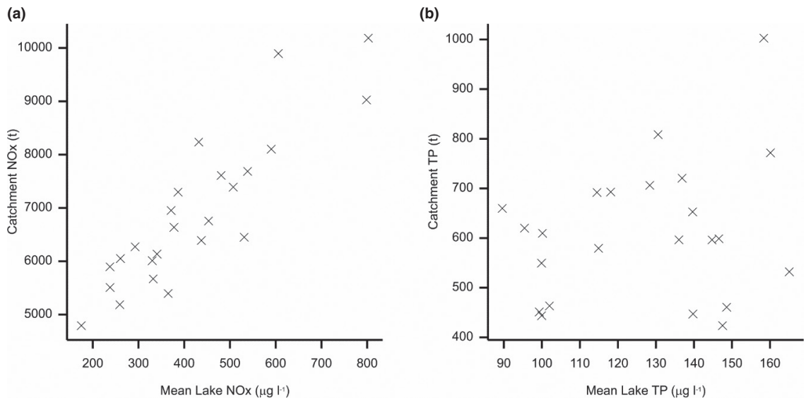
Fig. 4—Annual mean lake water concentration for total oxidised nitrogen (NO x ; µg/L) and catchment loading of NO x tonnes (T) per year (a) and annual mean lake water concentration for total P (TP; µg/L) and catchment loading of TP (T) per year (b).
