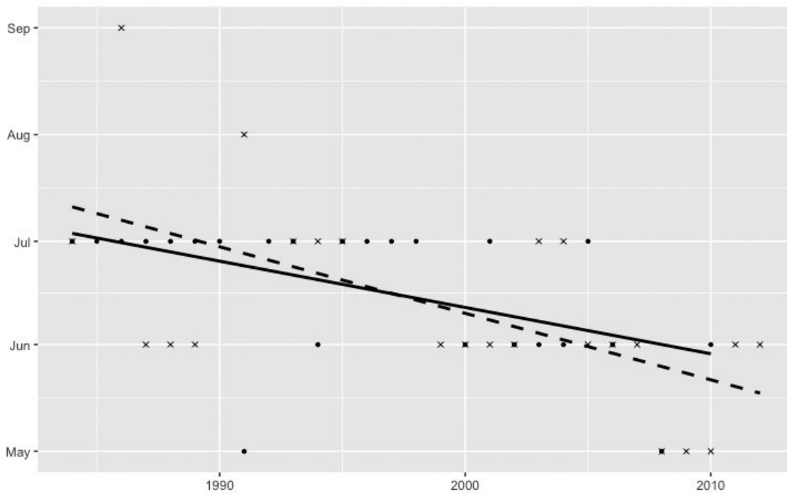
Fig 6— Temporal trends in commencement of total oxidised N ( \text{NO}_x ) depletion (concentration of \text{NO}_x < 0.06\text{mg/L} ) and soluble reactive P (SRP) sediment release (concentration of SRP was >10\mu\text{g/L} ), 1984–2012. The temporal trend of \text{NO}_x is represented by dots and the solid line, while that of SRP is represented by crosses and the dashed line.
