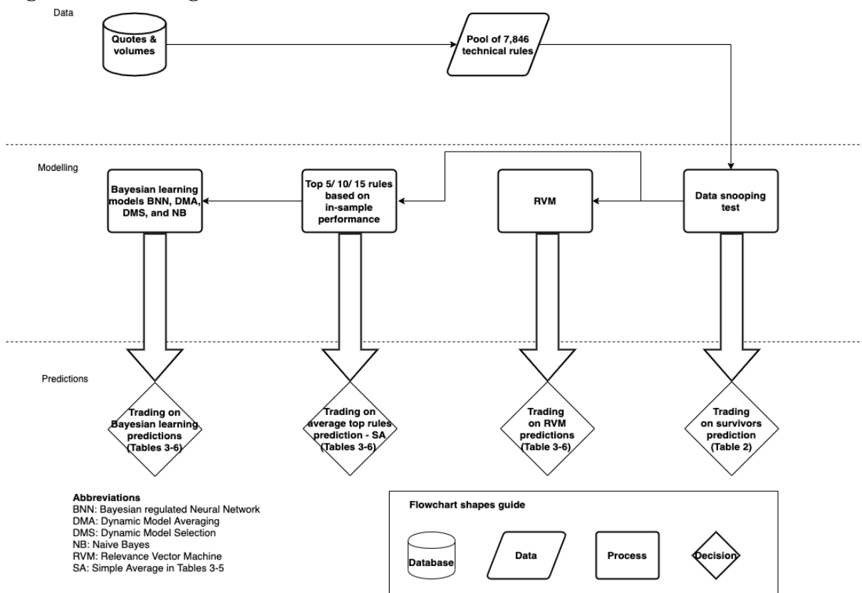
Figure 1: Modelling flowchart
