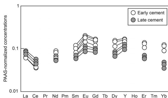
Fig. 6. Rare earth element and Y patterns of the Jebel Huwayyah Mound fluid conduit cements (early phase and late phase only). Data were normalized to post-Archaeon Australian shale (PAAS; Taylor & McLennan, 1985). Note that the data presented are averages of eight to ten laser-ablation spots (see online Supplementary Material Table S2).
