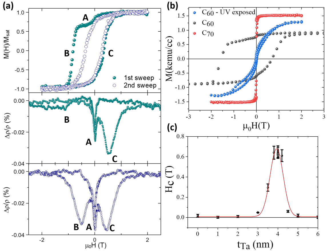
FIG. 4. (a) [Top], hysteresis loops obtained from the first and second sweeps after cooling a Co/ C_{60} bilayer in a 2 T applied field to 5 K. The exchange bias and asymmetry is completely destroyed after a single cycle. [Middle], AMR (anisotropic magneto-resistance) recorded during the first sweep. Note that the magnetoresistance, \Delta\rho , is zero at point B. [Bottom], AMR recorded during second sweep. Note that the AMR now exhibits expected behaviour for both forward and backward sweeps. (b) Comparison of hysteresis loops at 5 K for Co/ C_{60} bilayer (black), a Co/ C_{70} bilayer (red) and the same Co/ C_{60} bilayer after removing the molecular film with a combination of acetone and UV. (c) Dependence of the maximum recorded coercivity at 5 K on the thickness of the Ta seed layer, showing the importance of seeding the correct structure in the Co thin film.
