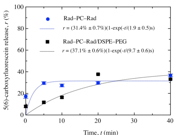
Figure 3. The release of 5(6)-carboxyfluorescein containing liposomes formulated from Rad-PC-Rad and Rad-PC-Rad/DSPE-PEG. The samples were heated to a temperature of 37 °C and kept at constant temperature for a period of 0, 5, 10, 20, and 40 minutes. The final spontaneous CF release was about 35%. The data are represented as mean values, error bars indicate standard deviation ( n = 5 ).
