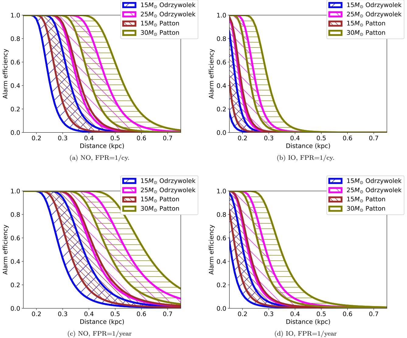
Figure 9. Expected maximum range of detection in the final 12 hours before collapse, for 15 M_{\odot} and 25 M_{\odot} stars. The width of the bands shows uncertainty due to levels of background in SK-Gd, and the difference between models of \gamma -ray emission from TNC on Gd.
