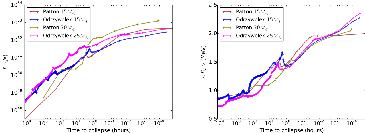
Figure 1. Comparison of L_\nu number, and \langle E_\nu \rangle mean energy, of emitted \bar{\nu}_e , against time to core collapse, in models by Odrzywolek & Heger (2010) and Patton et al. (2017b). Spikes in both quantities are caused by ignition of fusion of heavier isotopes in the core or shell of the star.
