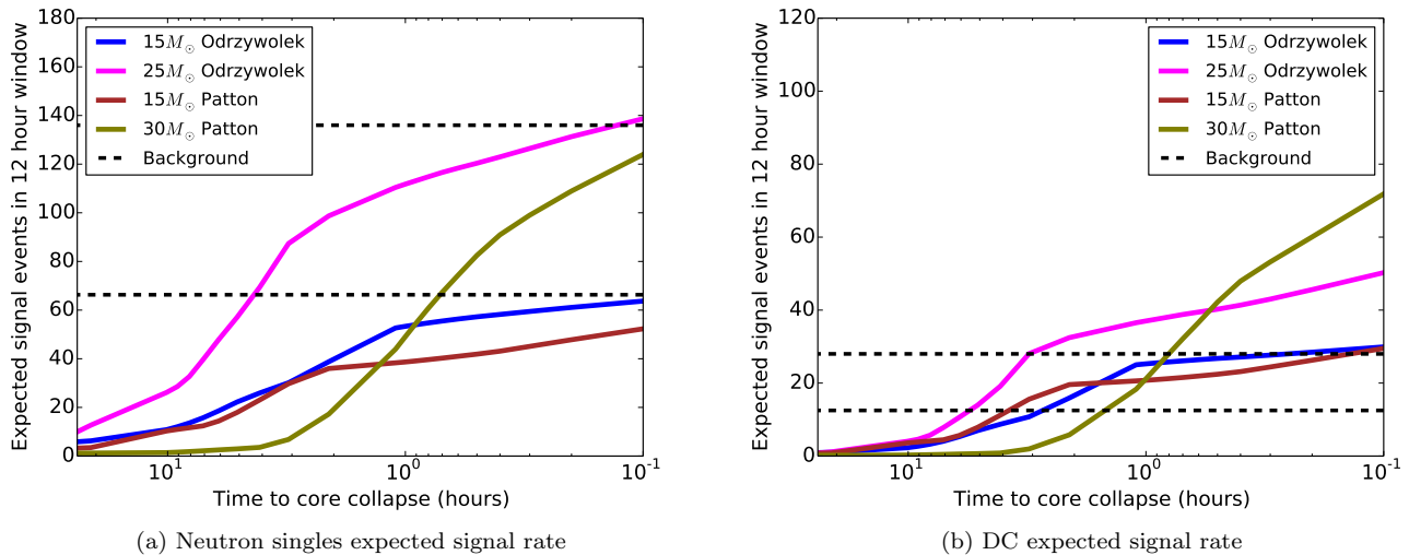
Figure 11. Expected signal events in 12 hour time window, after detection efficiencies are taken into account as per section 5. A distance of 200 pc and NO is assumed. Dotted lines show the high and low background assumptions.
