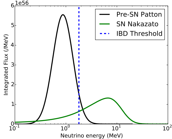
Figure 2. Total emission versus energy for \bar{\nu}_e from pre-SN and from a SN burst, integrated over the full time range of the respective models. The dotted line shows reaction threshold of IBD. Pre-SN spectrum shown is a 30 M_{\odot} model from Patton et al. (2017b) , SN spectrum is 30 M_{\odot} from Nakazato et al. (2013) . 30 M_{\odot} was chosen so that the two would have the same mass. Note that the pre-SN neutrinos are emitted over a much longer timescale (1000 hours vs. 20 seconds), and that the IBD cross section is strongly energy dependent.
