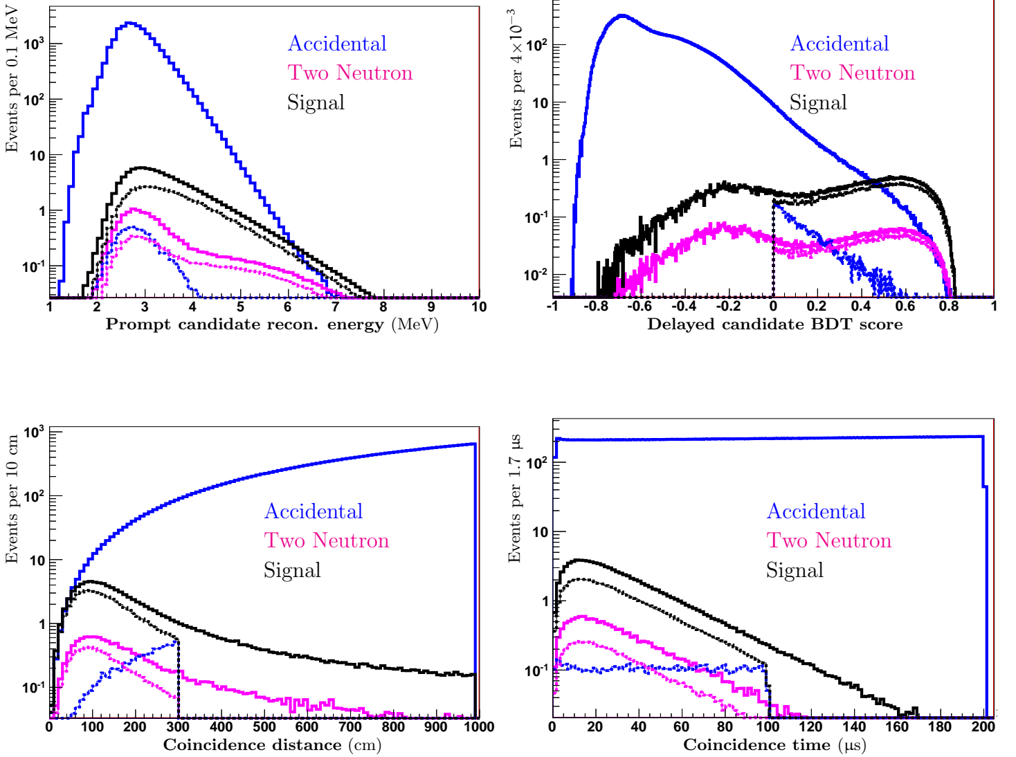
Figure 6. Distribution of DC channel variables in final selection for signal and largest backgrounds. Solid lines show before selection, dotted after. Background is normalised to 12 hours. Signal is normalised to the flux in the final 12 hours before CCSN for a 20 M_{\odot} star at 500 pc.
