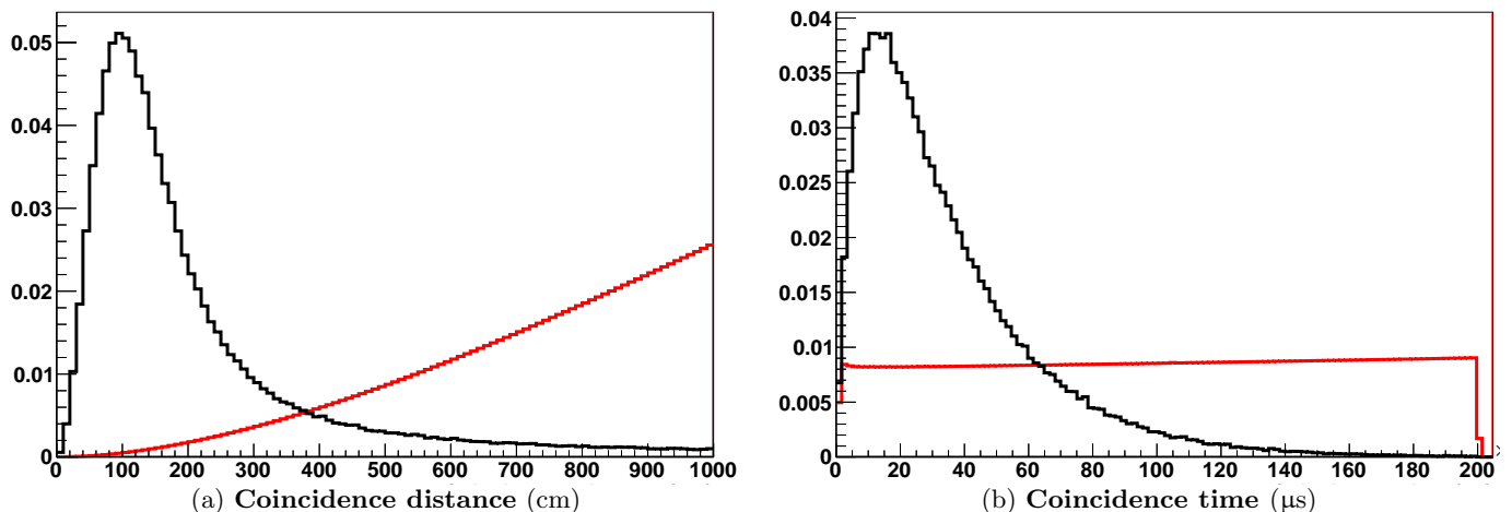
Figure 5. Distribution of the reconstructed distance (a) and reconstructed time (b) between simulated event candidates (with 3 MeV prompt positrons) before selection. Signal MC is shown in black and accidental background from data in red, area normalised to one.
