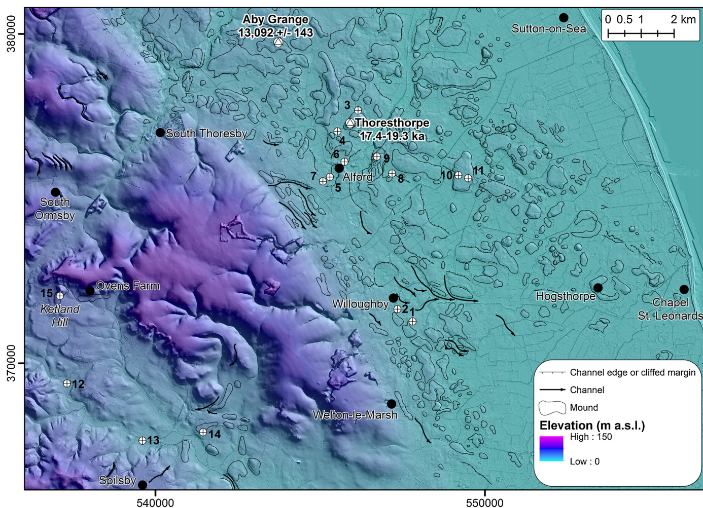
Fig. 5. Large scale geomorphology map for the area around Thoresthorpe on the Lincolnshire Marsh. Locations of selected borehole records are the numbered cross in circle symbols. Dated sites are triangle in circle symbols.
