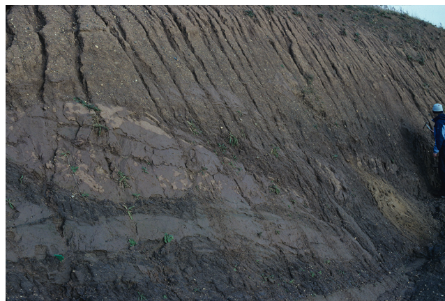
Fig. 4. Exposure through the glaciectonised rhythmites folded into the Marsh Till and sampled for OSL dating at Welton le Wold.
