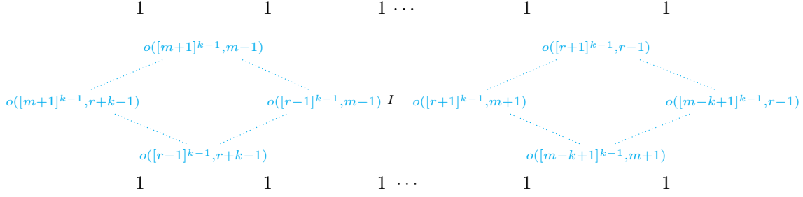
FIGURE 2. Ext-hammock of M_I where I = o([r]^{k-1}, m)
