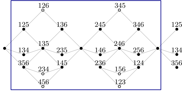
FIGURE 4. Auslander-Reiten quiver of \mathcal{C}(3,6) . Projective-injectives are drawn as white circles.
