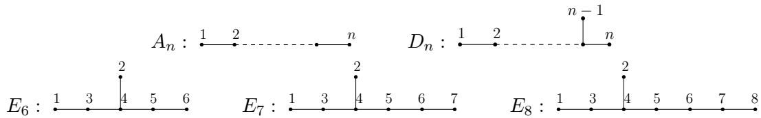
FIGURE 7. The Dynkin diagrams \Gamma_{\mathcal{C}} of the finite type cluster categories
