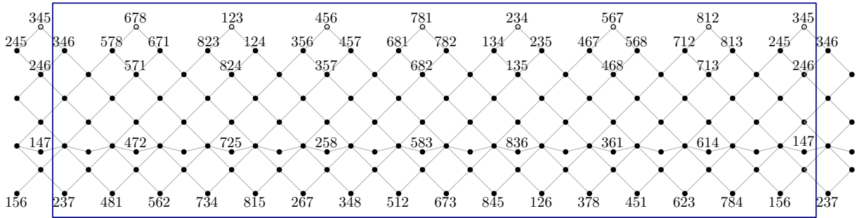
FIGURE 6. Auslander-Reiten quiver of \mathcal{C}(3, 8) .
