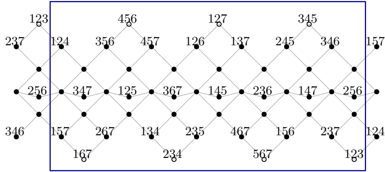
FIGURE 5. Auslander-Reiten quiver of \mathcal{C}(3, 7) .
