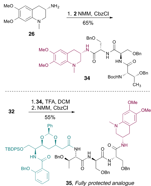
Scheme 11 Coupling experiments.
