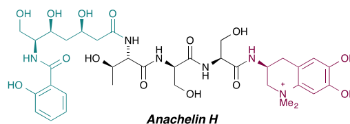
Figure 1. Structure of anachelin H , highlighting the three fragments.
