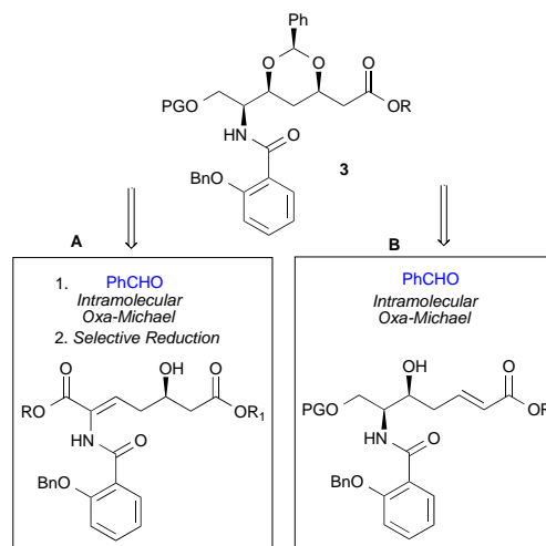
Scheme 2 Retrosynthetic analysis for polyketide fragment.
