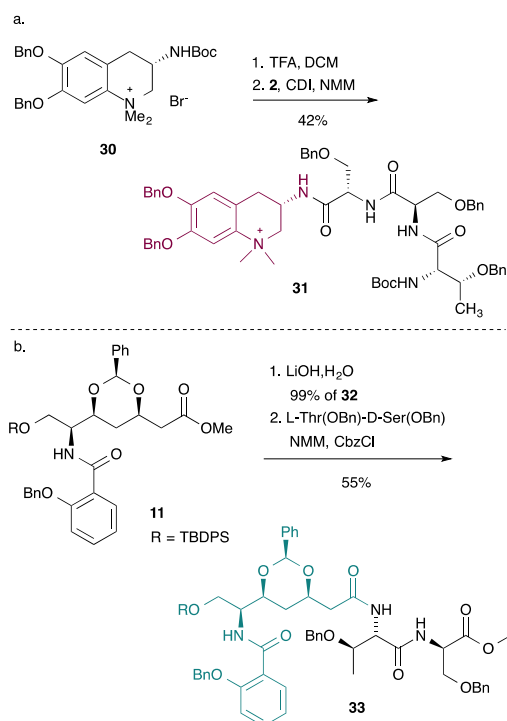
Scheme 10 Coupling experiments.
