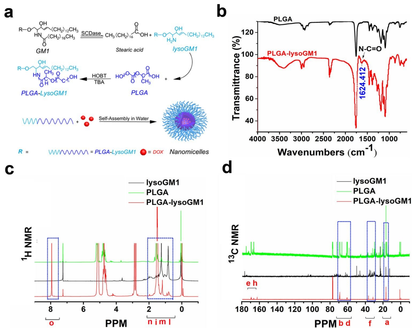
Fig. 1 Synthesis and Characterization of PLGA-lysoGM1. (a) A schematic diagram of PLGA-lysoGM1/DOX micelles formation. (b) The FTIR spectrum of the synthesised PLGA-lysoGM1 sample. (c) The 1 H NMR spectrum of PLGA-lysoGM1. (d) The 13 C NMR spectrum of PLGA-lysoGM1.
